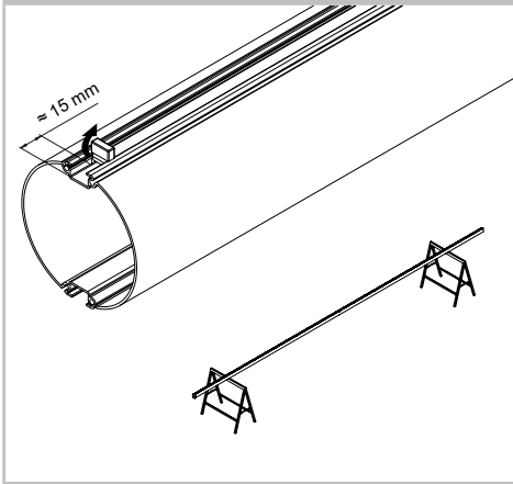
Fig. 6 - UPPER LED
